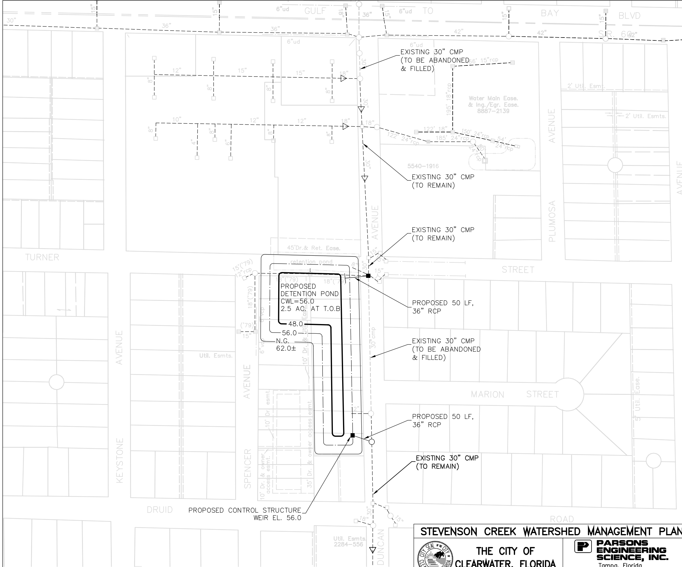
FIGURE 3.1-34 PROJECT 7B DUNCAN AVENUE/TURNER STREET DETENTION POND
