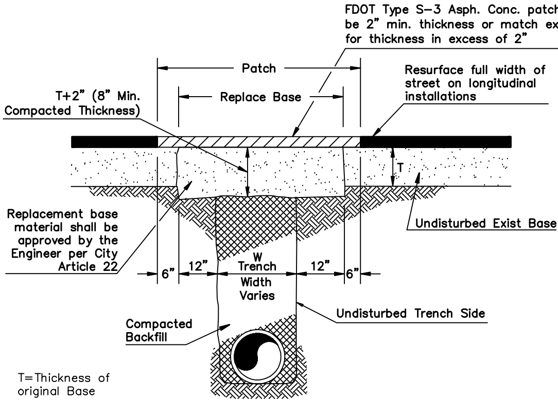
ASPHALT STREET AND DRIVEWAY REPLACEMENT REQUIRED FOR UTILITY CONSTRUCTION
