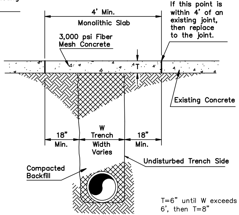
CONCRETE REPLACEMENT REQUIRED FOR UTILITY CONSTRUCTION
