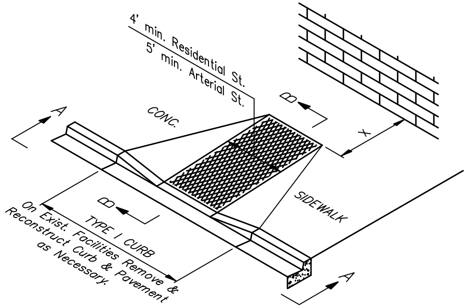
ISOMETRIC VIEW
