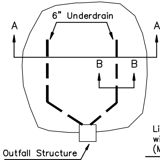
DETENTION POND
